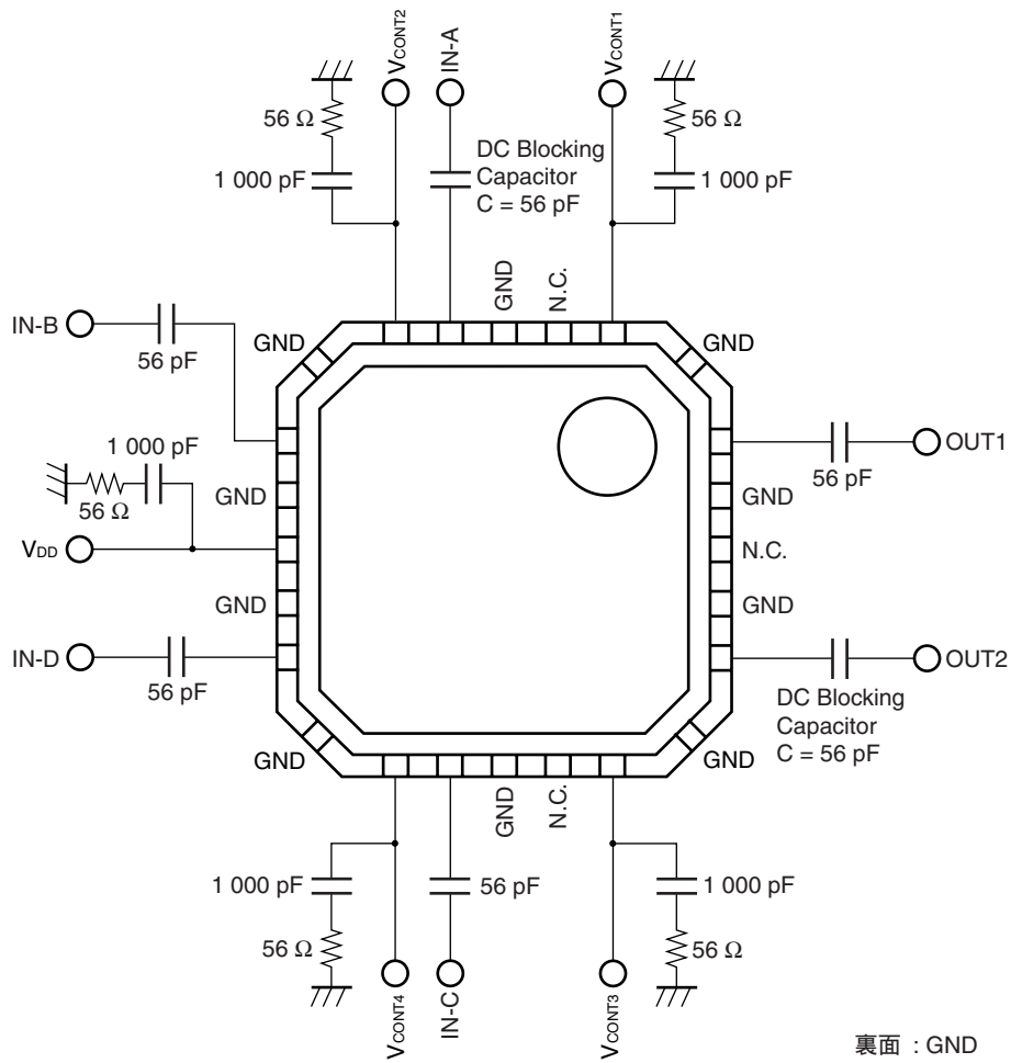
評価回路図 ( V_{DD} = +5.0\text{ V} , V_{CONT} = +5.0\text{ V/0 V} , Z_o = 50\ \Omega )
