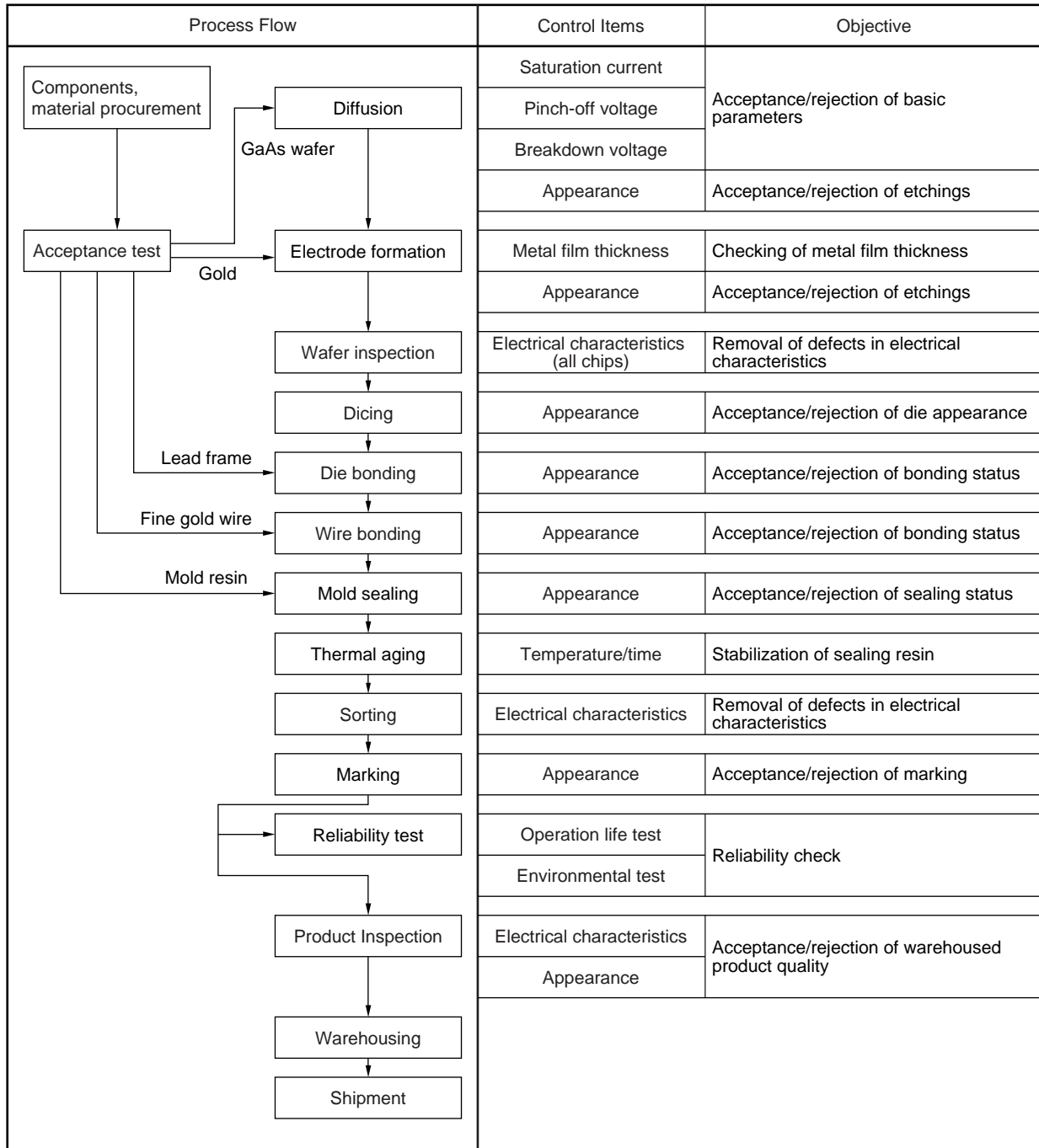
Figure 2-3 An example of production process control flowchart of Power GaAs FET (plastic package)
