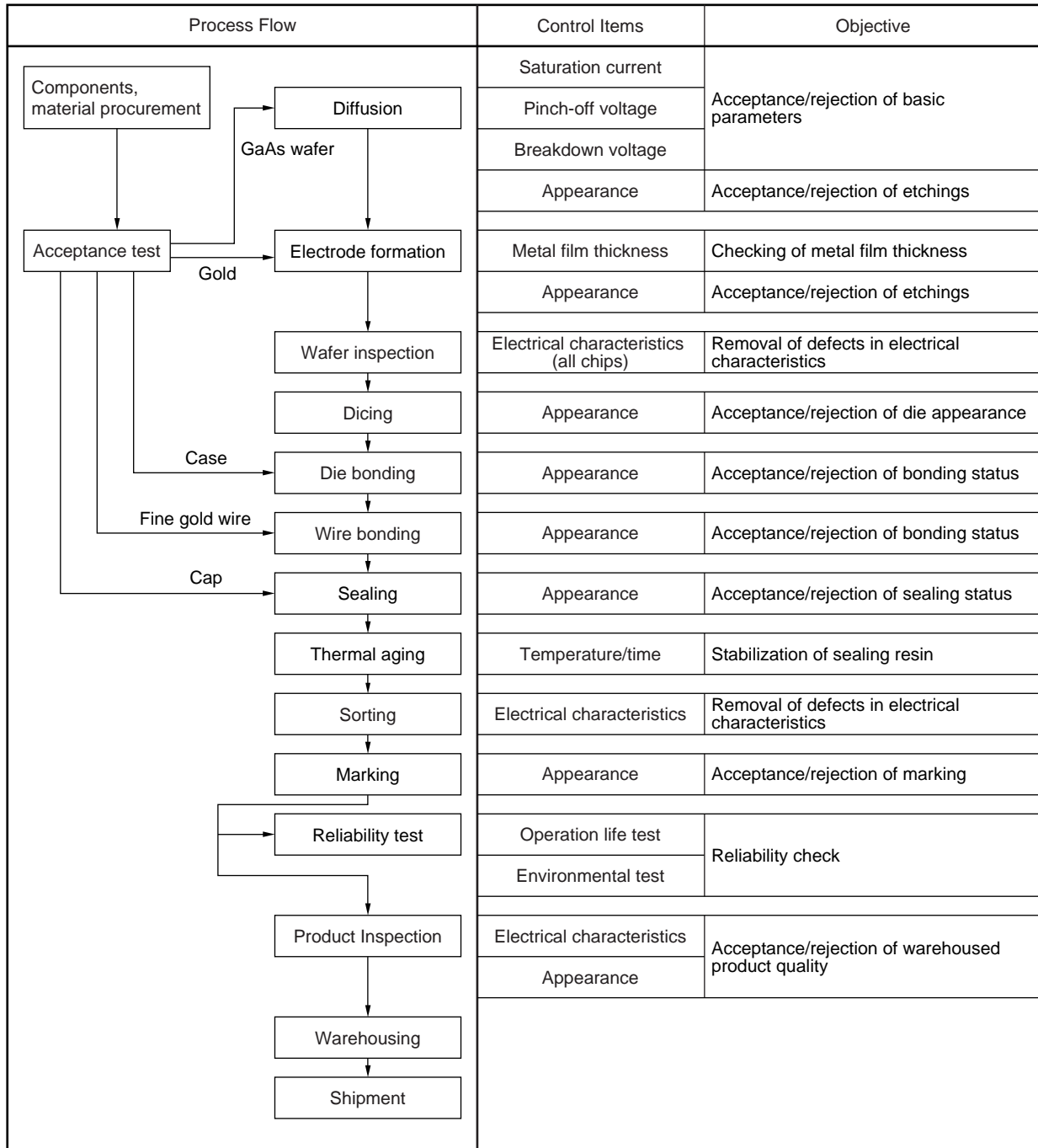
Figure 2-2 An example of production process control flowchart of Power GaAs FET (hollow plastic package)
