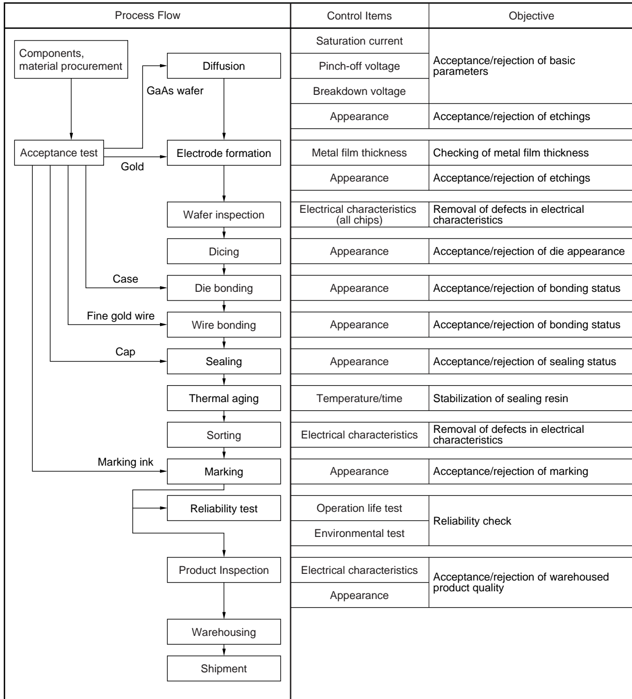
Figure 2-1 An example of production process control flowchart of Power GaAs FET (ceramic package)
